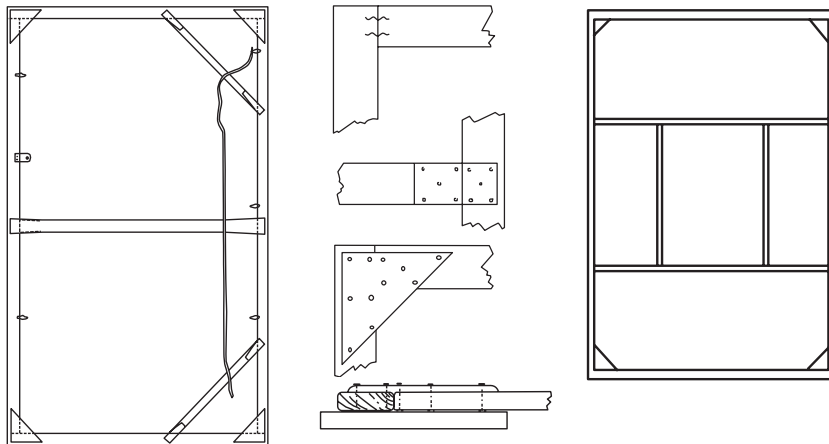
The flat on the left is plain and basic; the flat on the right is designed to include a window. Joints can be reinforced in several ways, as shown by the middle illustration.
