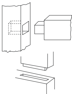
For extra strength, a flat can be assembled using mortise and tenon joints.
