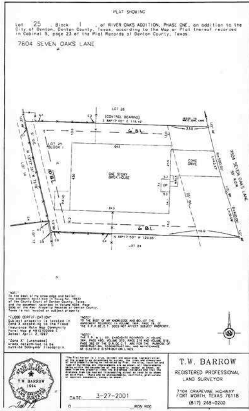
Boundary map with metes and bounds description
