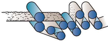
On the paper machine, a vacuum pulls water through the bottom of the forming fabric. The paper machine also has presses—rollers—that squeeze water out of the paper.
